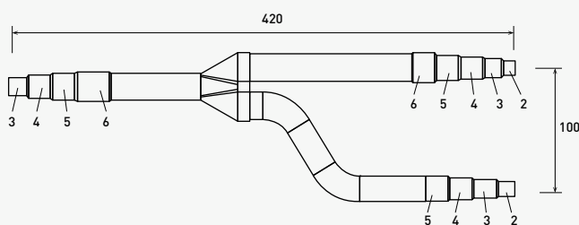
Gas piping
