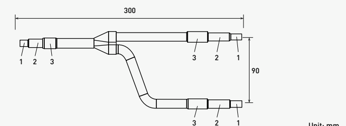
Liquid piping
