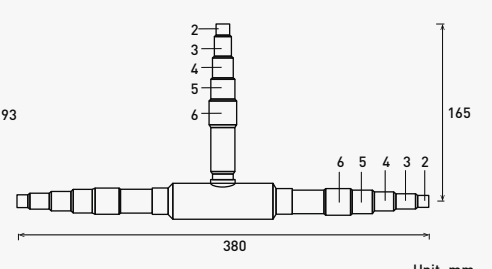
Liquid piping
