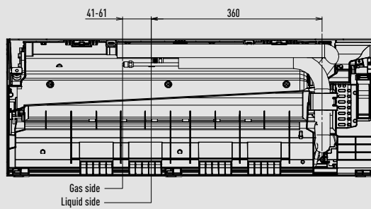
Relative position between the indoor unit and the installation plate
