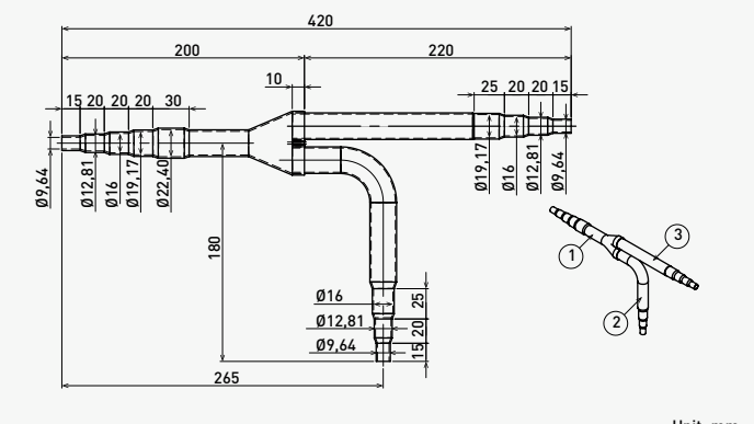
Liquid piping
