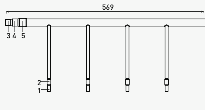
Size of connection point on each part (shown are inside diameters of piping)
